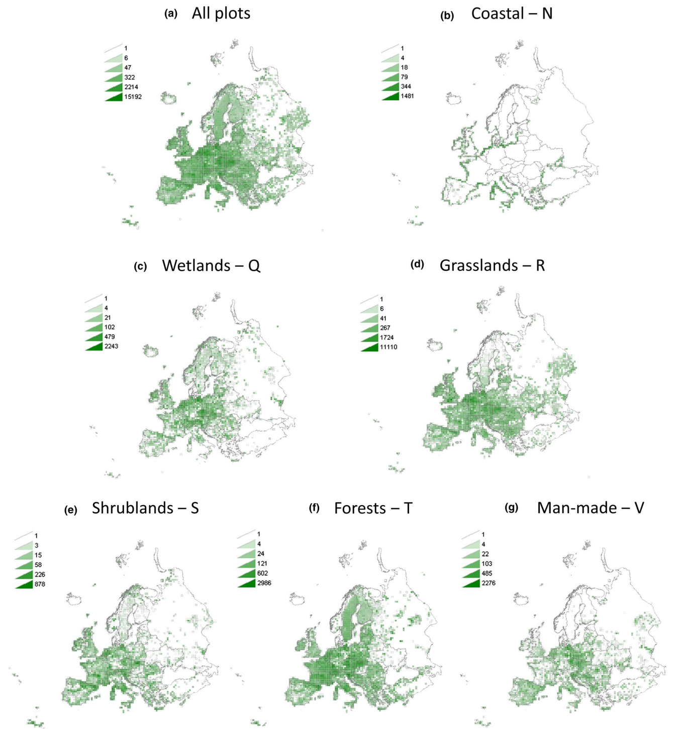
FIGURE 2 The density of the vegetation-plot data expressed as numbers of plots in 50 km × 50 km grid cells of the 1,261,373 plots used for the classification (a) and the plots classified by the expert system to habitat groups N, Q, R, S, T, V (b–g) and individual habitats within these groups [Colour figure can be viewed at wileyonlinelibrary.com ]
