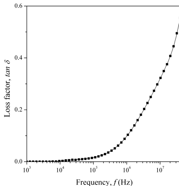
Fig. 14. The loss factor, \tan \delta of bulk FeSi/PFRSiO 2 composite core.
