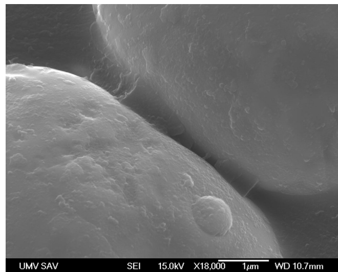
Fig. 10. SEM image of two FeSi particles coated and stuck together by PFRSiO 2 inside FeSi/PFRSiO 2 sample.
