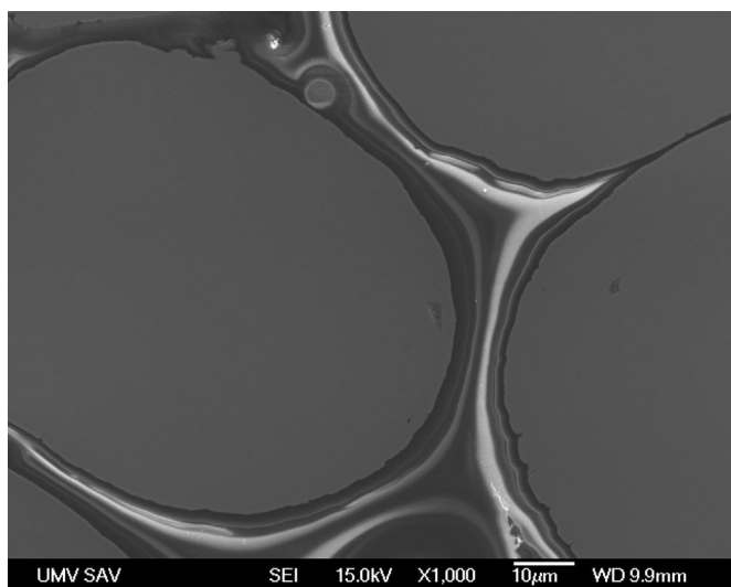
Fig. 9. SEM image of the resin distribution around FeSi particles.
